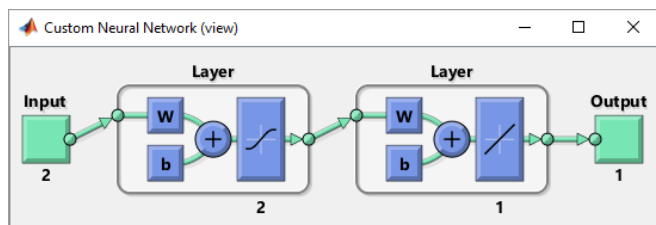
Figure 7: Architecture of back propagation neural network.
