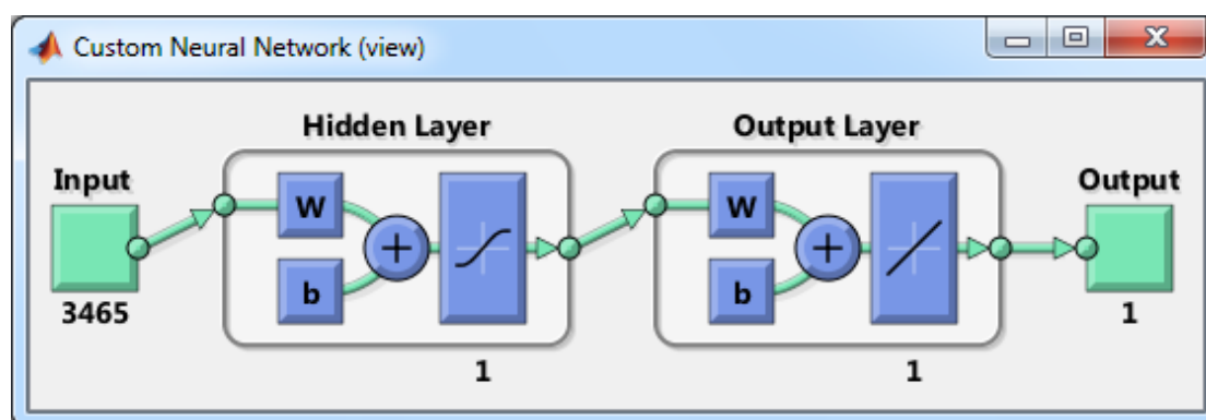
Figure 3.2. Architecture of back propagation artificial neural network
