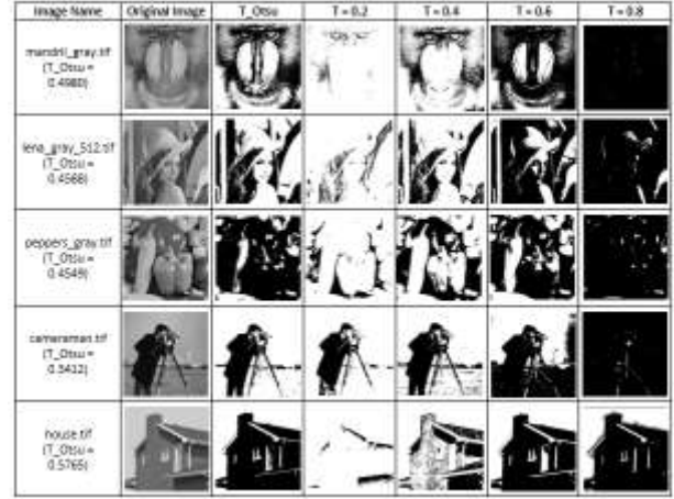
FIGURE 1. Application Otsu's method on thresholding process
